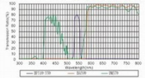
G激發光波濾色組件 Green Excitation
