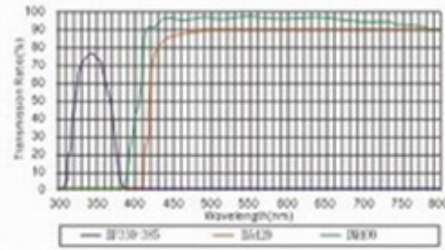
U激發光波濾色組件 Ultraviolet Excitation
