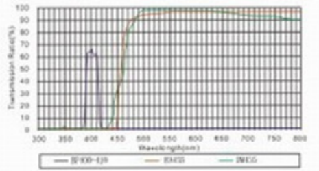
V激發光波濾色組件 Violet Excitation
