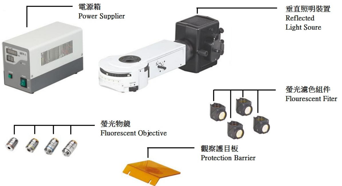
FOR MD-600 Fluorescent Attachment
